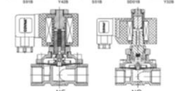
HK02/02K/31/32/41 Direct acting 1/8-1/2 2W NC/NO
